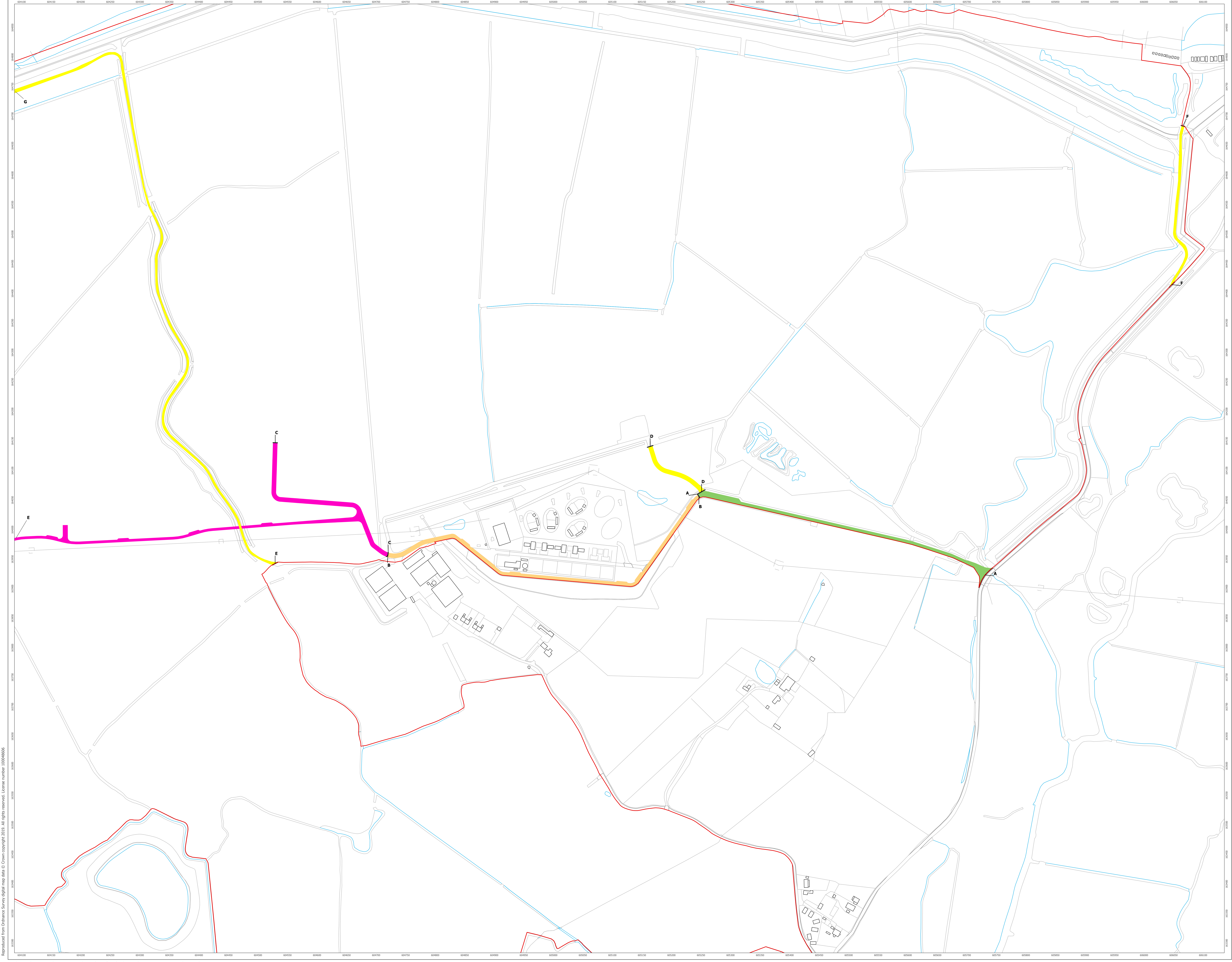
Streets and Access Plan - East Figure 3
